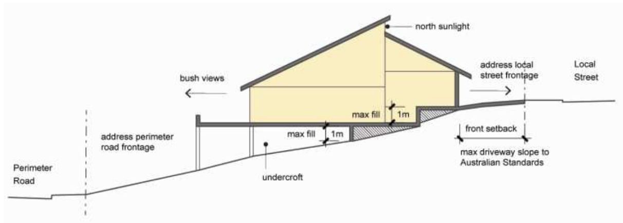
Figure 13: Sloping site
